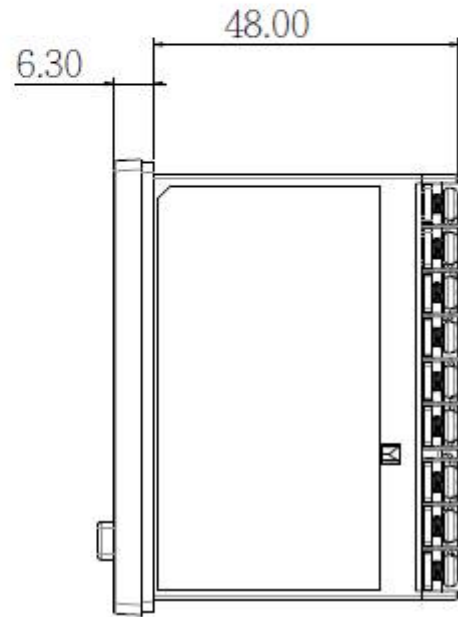
2-10. ZEL-C72 Dimension without Clamp
