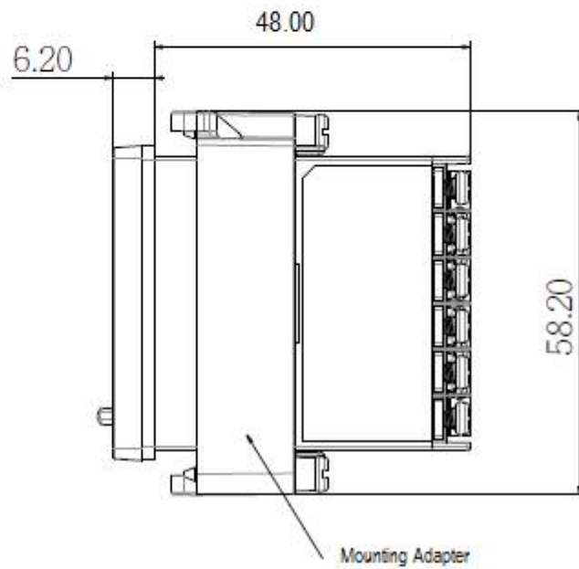
2-3. ZEL-C62 Dimension with clamp
