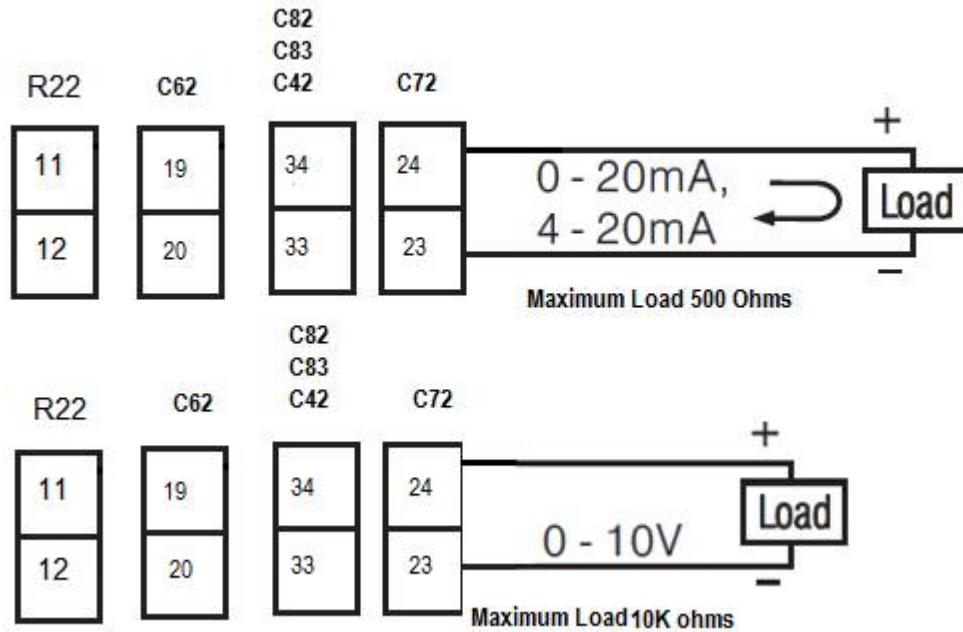
2-43. Retransmission Wiring
