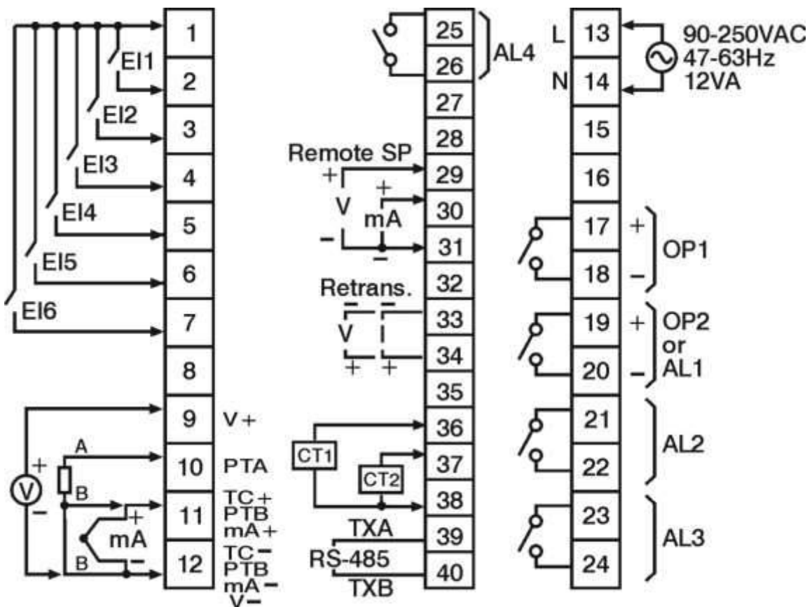
2-20. ZEL-C82 & ZEL-C42 Rear Terminal Connection
