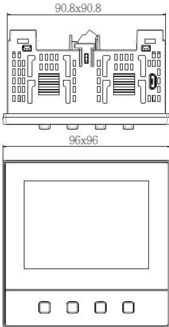
2-12. ZEL-C42 Dimension without Clamp
