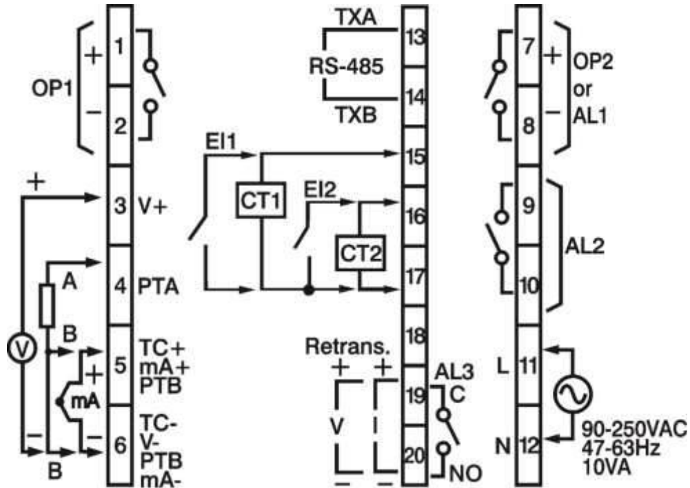
2-19. ZEL-C62 Rear Terminal Connection
