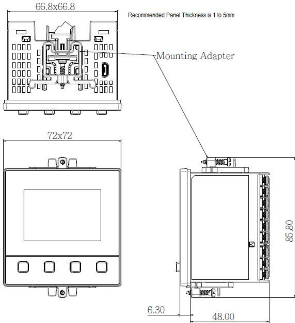
2-9. ZEL-C72 Dimension with Clamp
