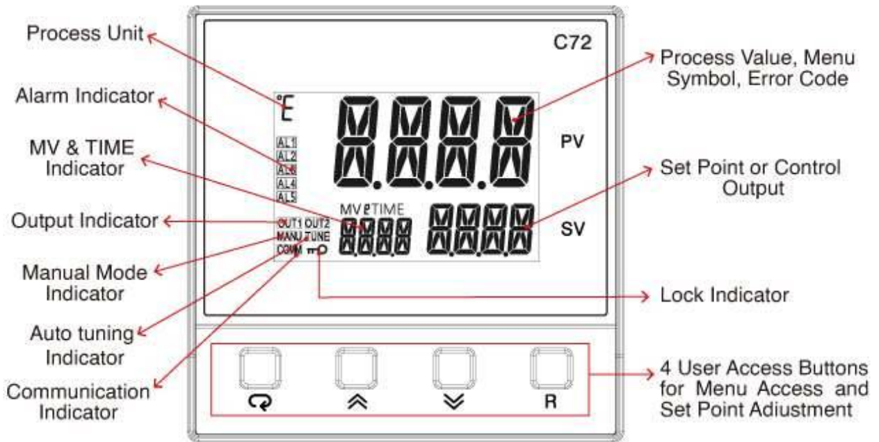
1-9. ZEL-C72 Front Panels Keys and Display
