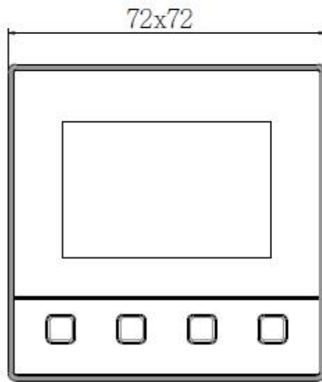
2-10. ZEL-C72 Dimension without Clamp
