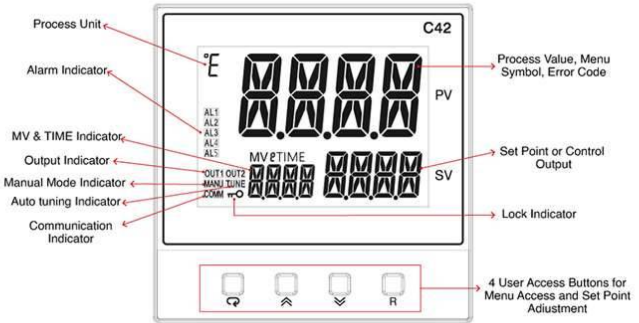
1-10. ZEL-C42 Front Panel Keys and Display
