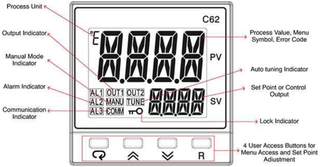
1-6.C62 Front Panel Keys and Display
