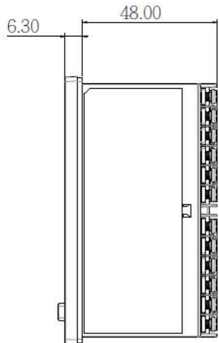
2-12. ZEL-C42 Dimension without Clamp
