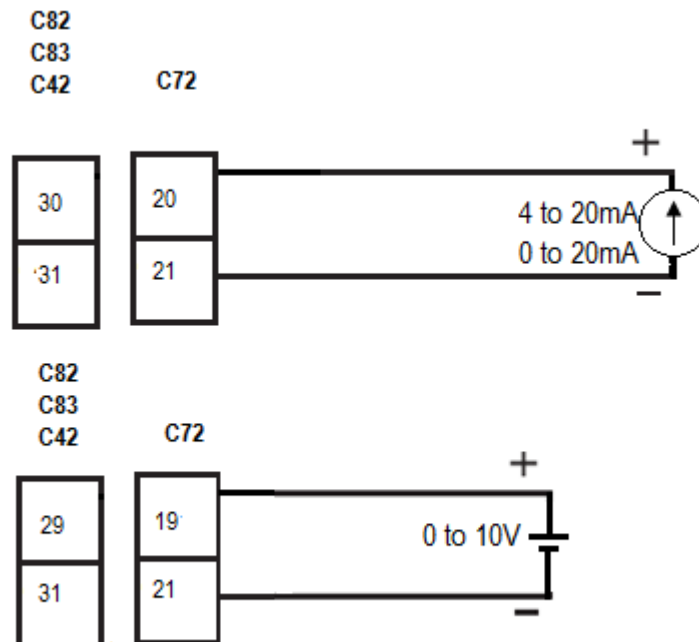
2-44. Remote SetPoint
