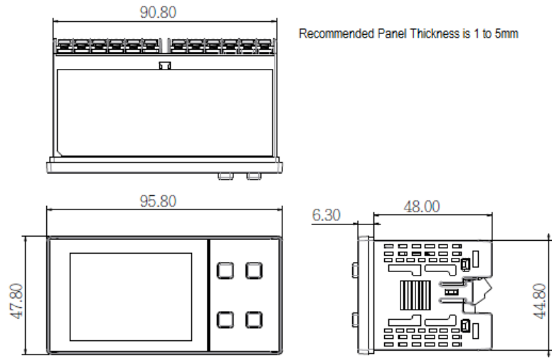
2-8. ZEL-C83 Dimension without Clamp
