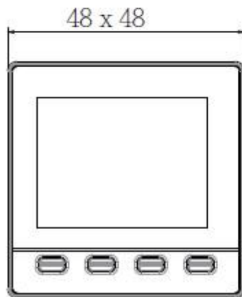
2-4. ZEL-C62 Dimension without Clamp
