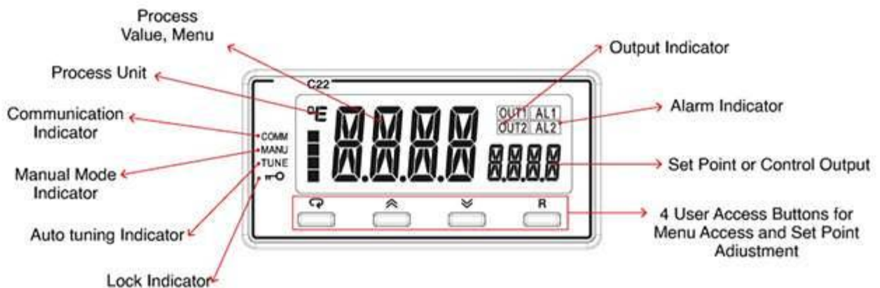
1-5. ZEL-C22 Front Panel Keys and Display
