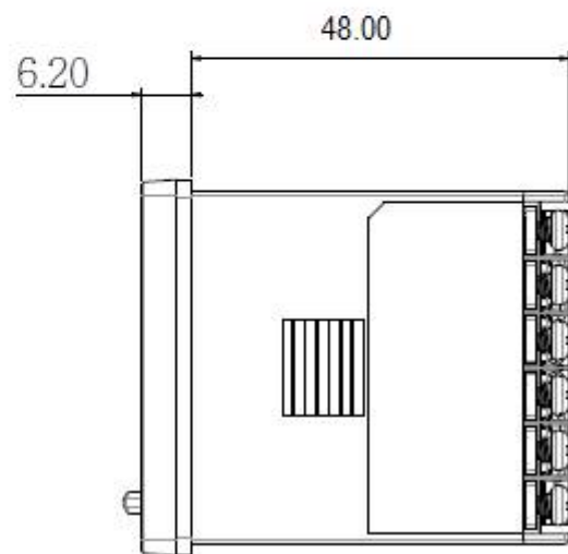
2-4. ZEL-C62 Dimension without Clamp
