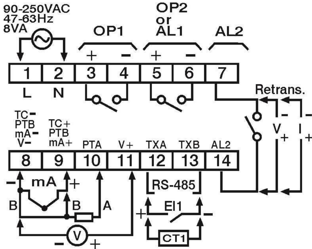
2-18. ZEL-C22 Rear Terminal Connection
