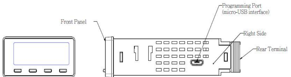
2-2. ZEL-C22 Dimension without Clamp
