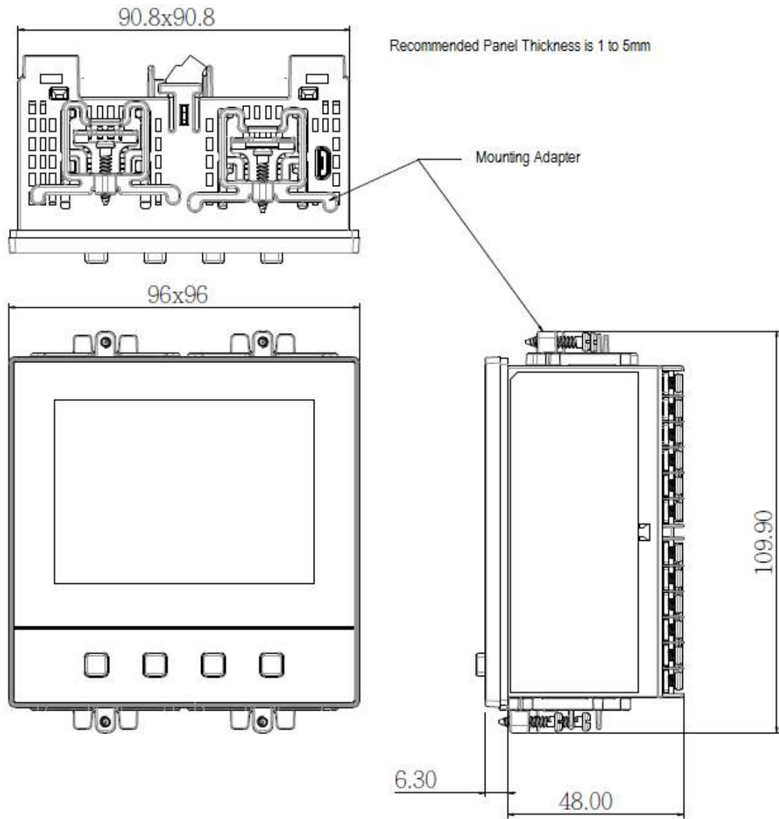
2-11. ZEL-C42 Dimension with Clamps
