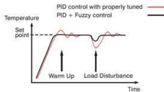
1-1.Fuzzy PID Control
