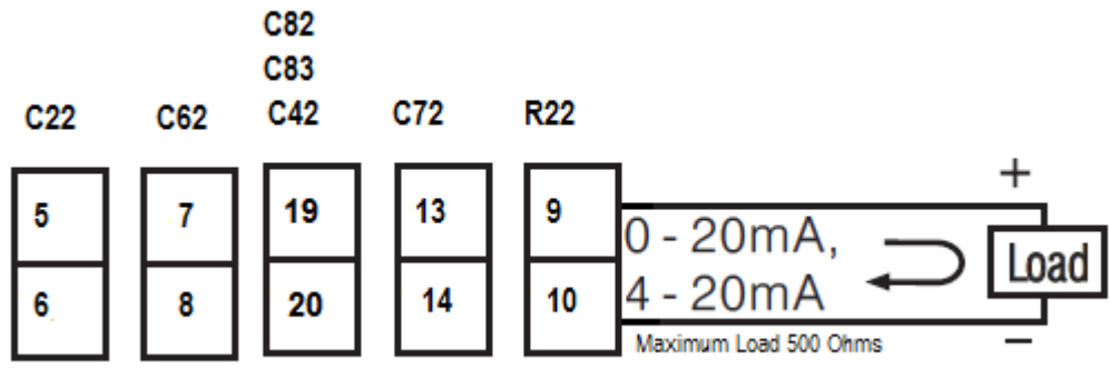
2-34. Output 2 Linear Current Control
