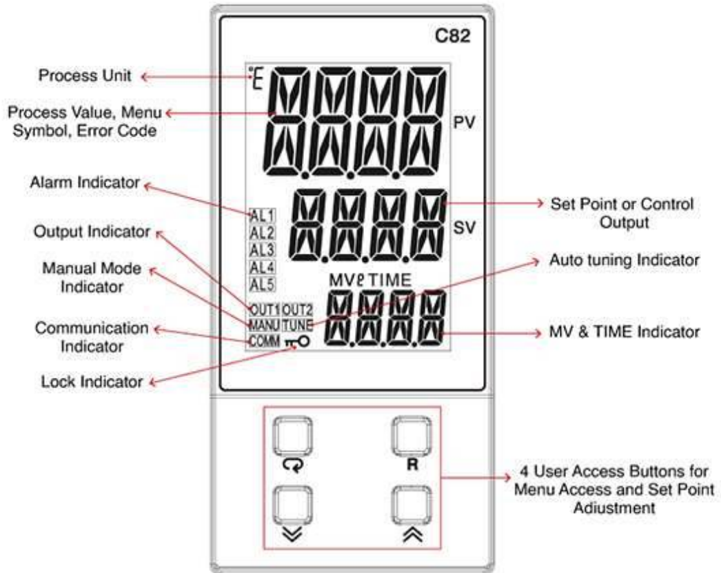
1-7. ZEL-C82 Front Panel Keys and Display
