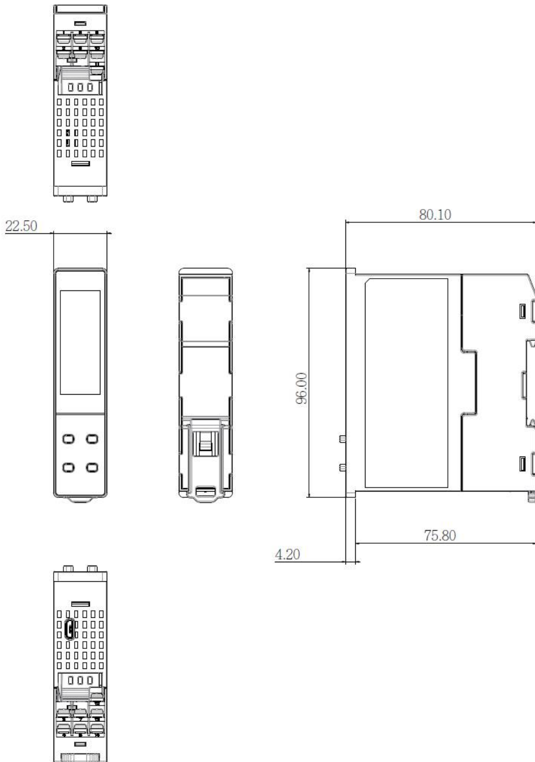
2-13. ZEL-R22 Dimension
