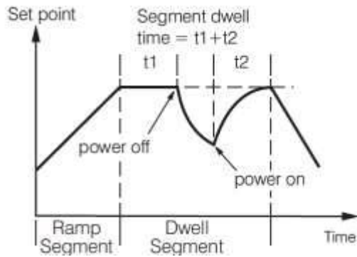
3-27. Power failure recovery from the profile at Dwell segment
