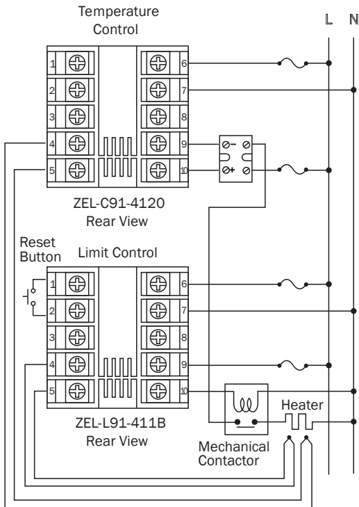
Figure 4-1 High Temperature Protection with Remote Reset
