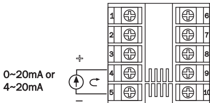
Figure 2.8 Linear Current Input Wiring
