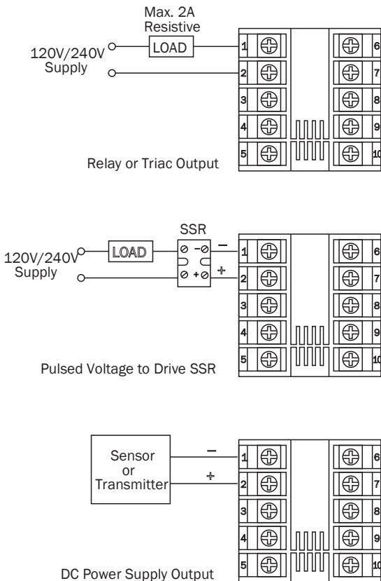
Figure 2-11 Output 2 Wiring
