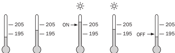
Figure 3.4 Latching Process Alarm
