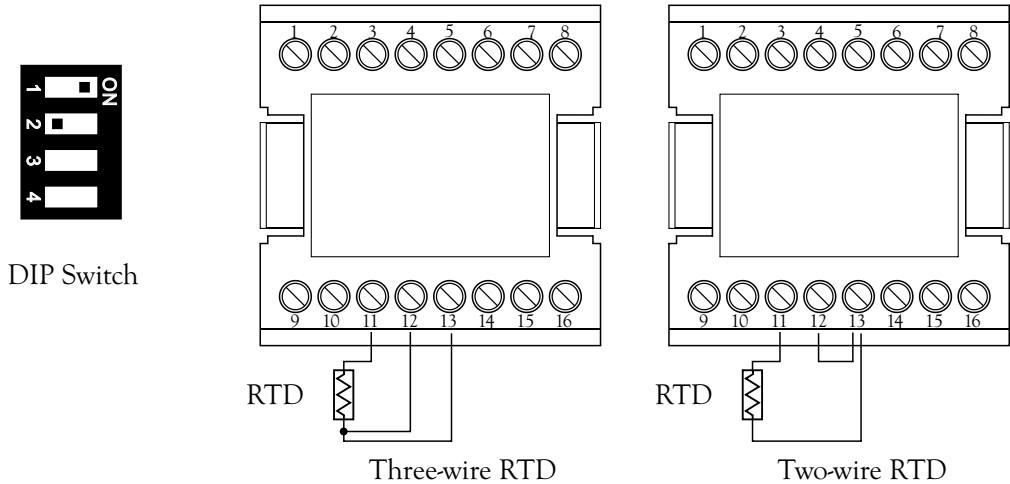
Figure 2.6 RTD Input Wiring
