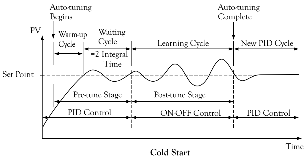
Figure 3.22 Auto-tuning Procedure
