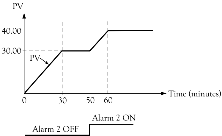
Figure 4.3 Ramp Accompanied with a Dwell Timer
