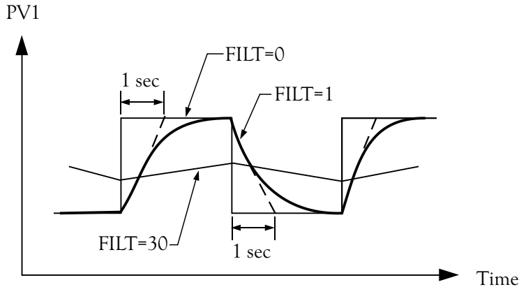
Figure 4.7 Filter Characteristics
