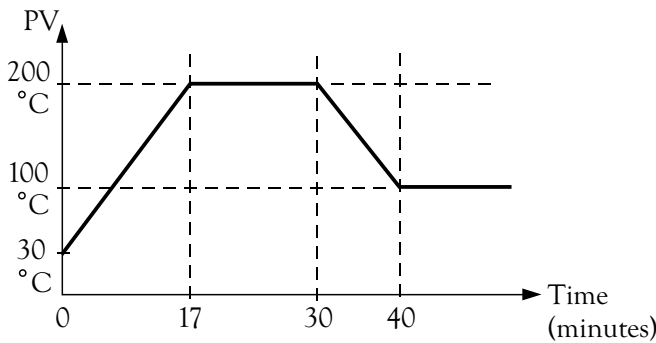
Figure 4.1 RAMP Function
