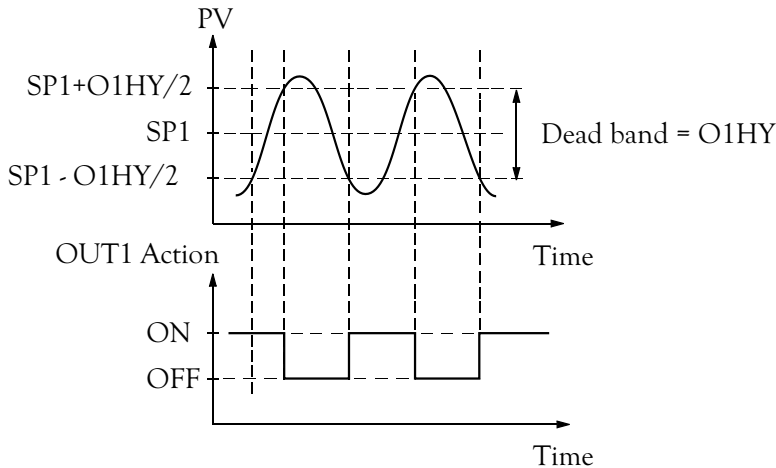
Figure 3.2 Heat Only ON-OFF Control
