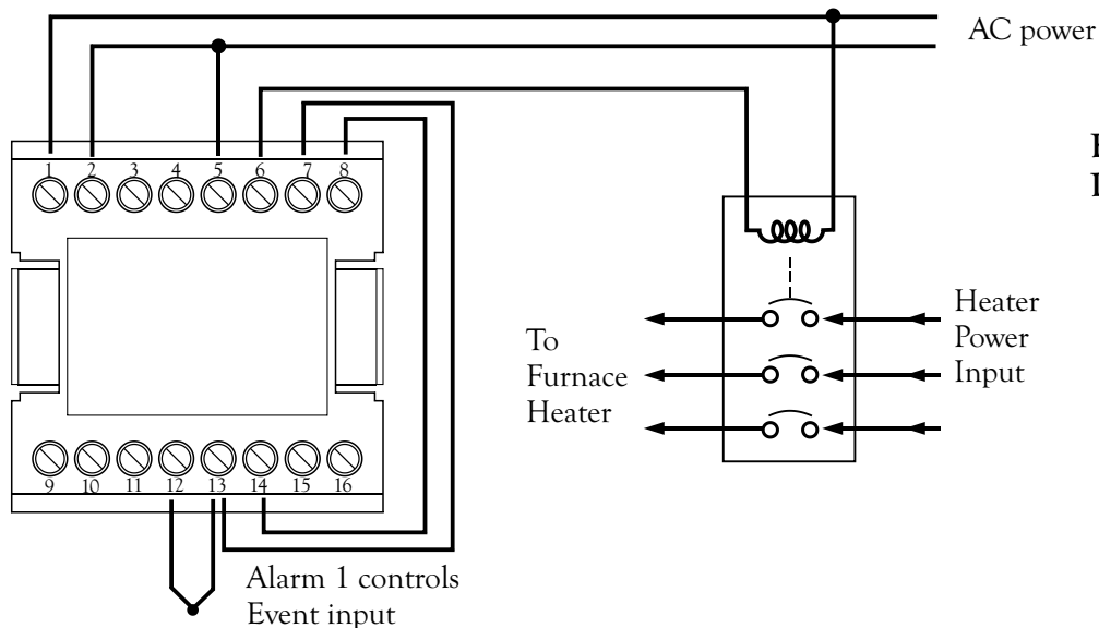
Figure 5.15 Dual PID Crossover
