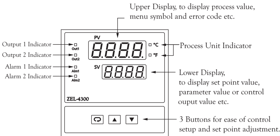
Figure 1.4 Front Panel Description
