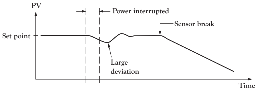
Figure 3.21 Benefits of Bumpless Transfer
