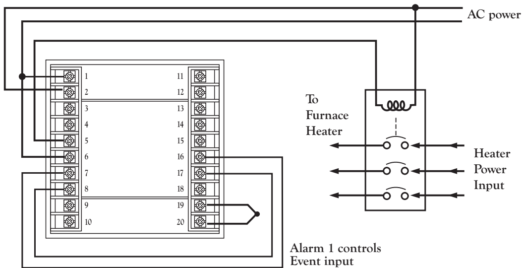
Figure 5.14 Dual PID Furnace
