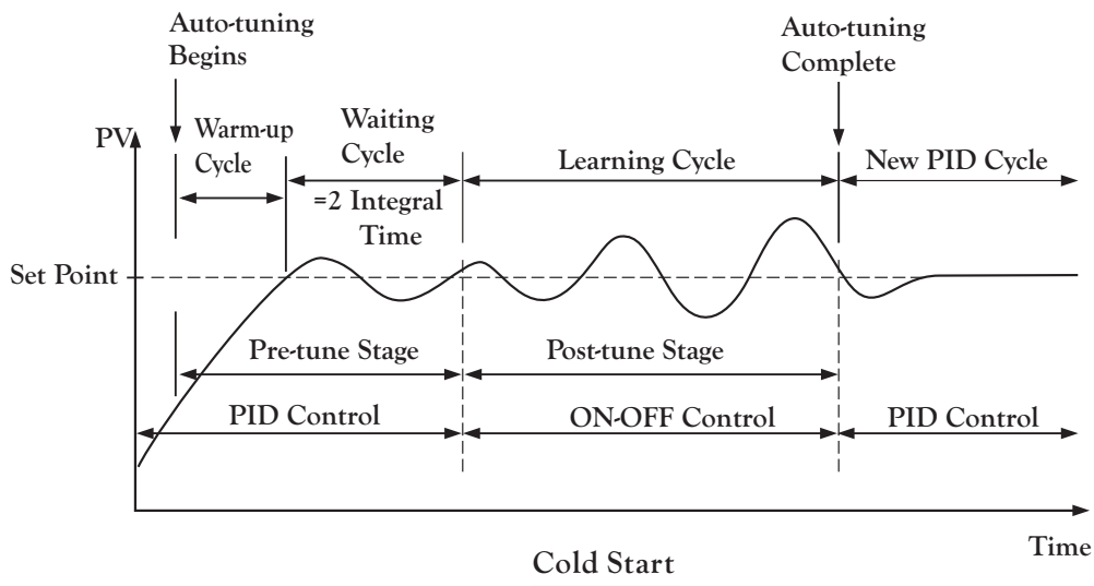
Figure 3.22 Auto-tuning Procedure
