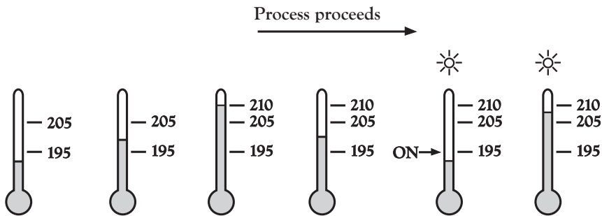
Figure 3.8 Latching / Holding Process Alarm
