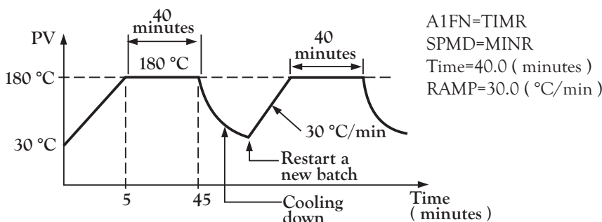
Figure 5.11 Temperature Profile of Baking Oven
