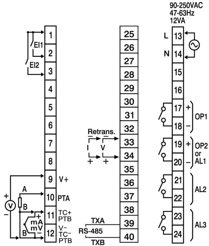
2-7 ZEL-L42 Rear Terminal Connection – High Voltage Input Power
