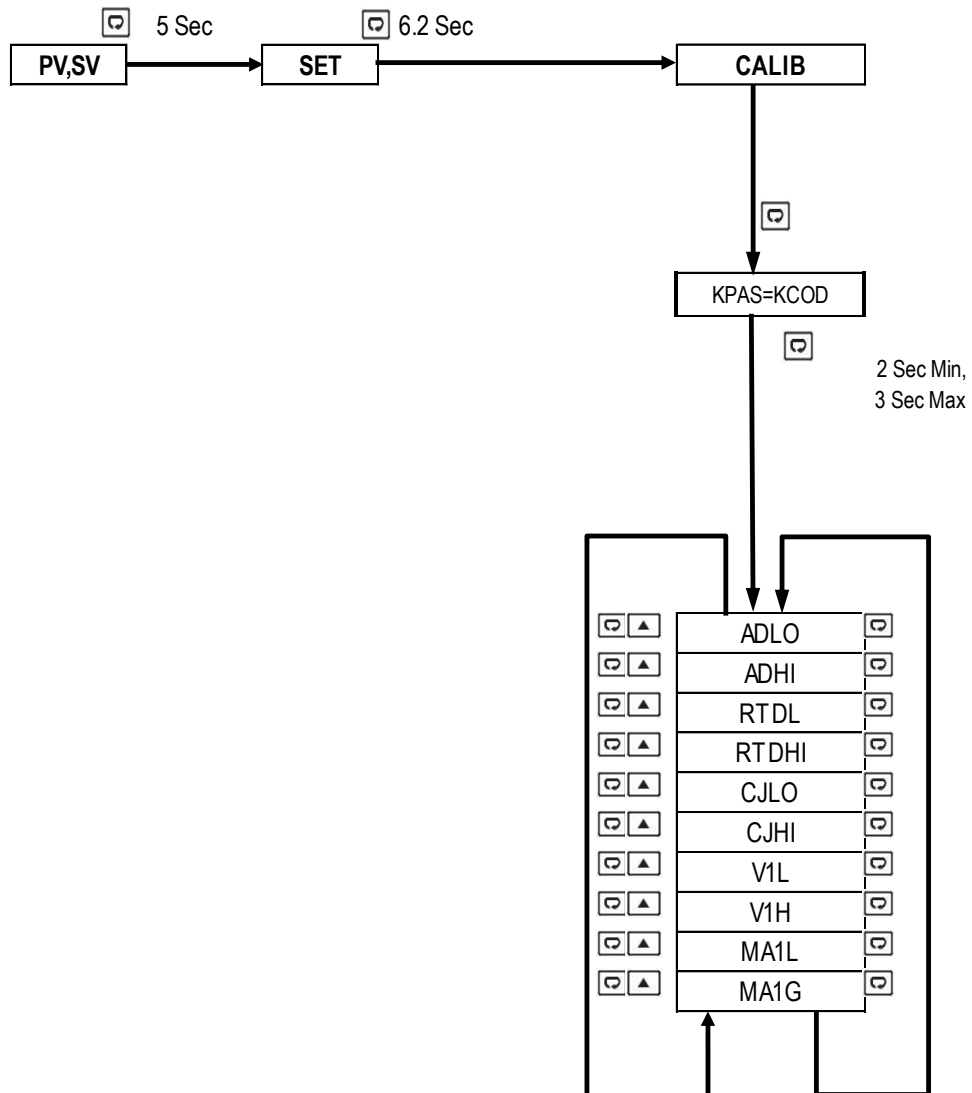
1-8 Calibration Menu
