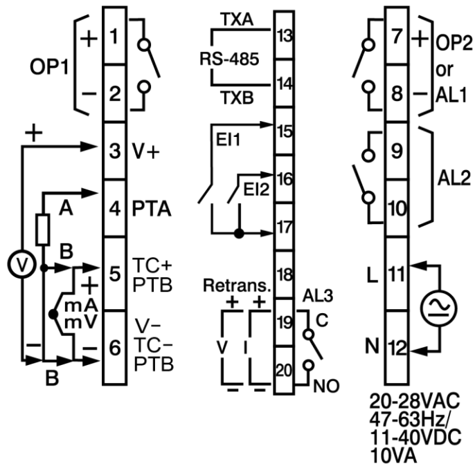
2-10 ZEL-L62 Rear Terminal Connection – Low Voltage Input Power
