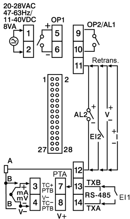
2-12 ZEL-L22 Terminal Connection– Low Voltage Input Power
