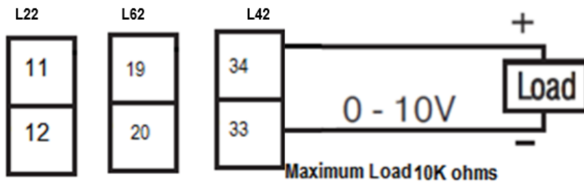
2-25 Retransmission Wiring - Voltage
