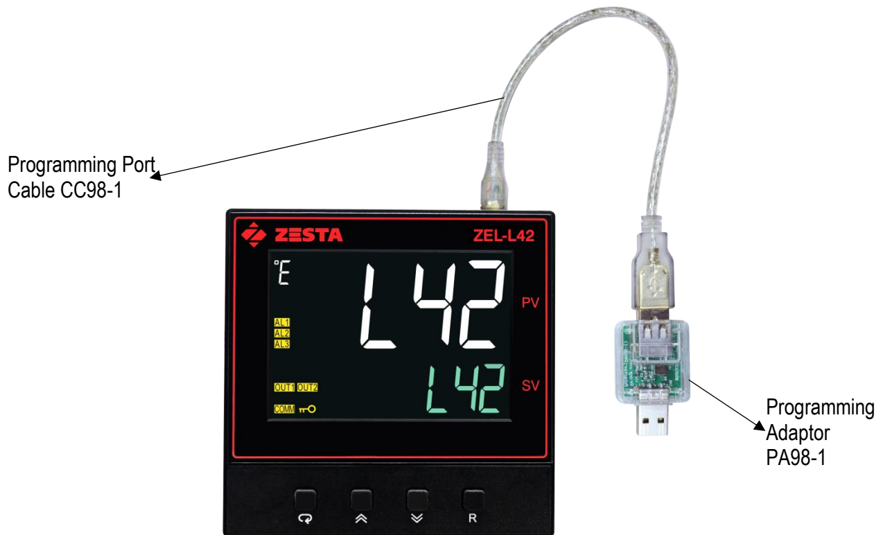
1-2 Programming Port Connection with Programming Port Adaptor
