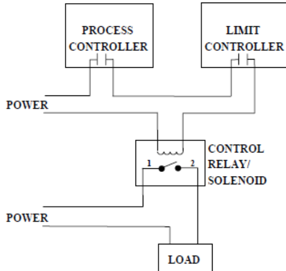
Incorrect Wiring
