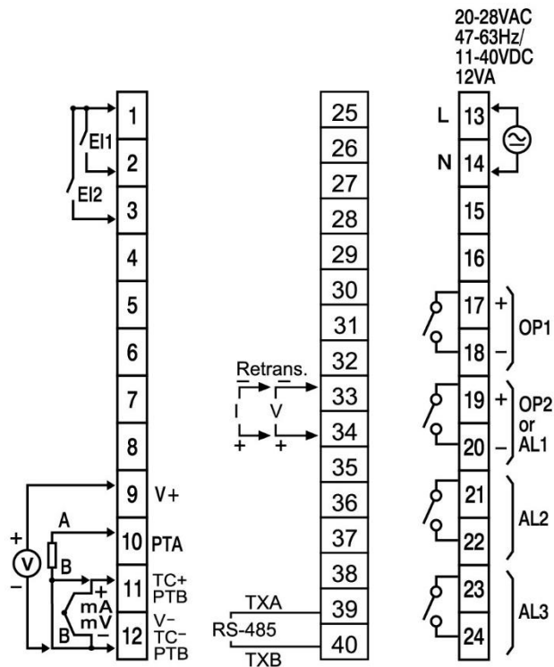
2-8 ZEL-L42 Rear Terminal Connection – Low Voltage Input Power
