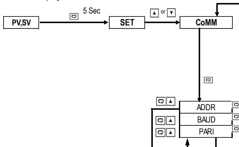
1-11 Communication Menu
