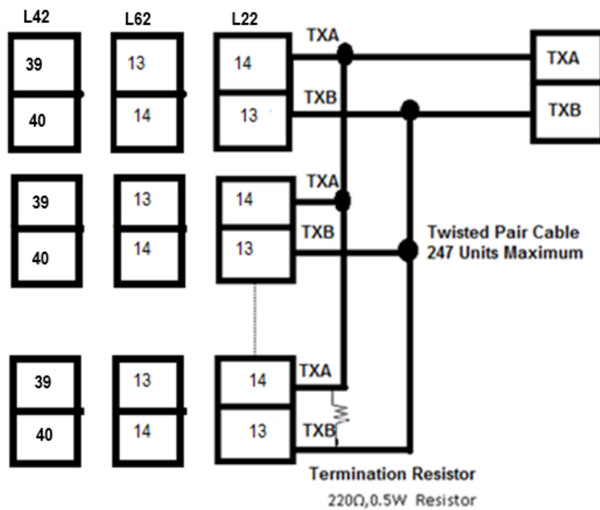
2-26 RS-485 Wiring
