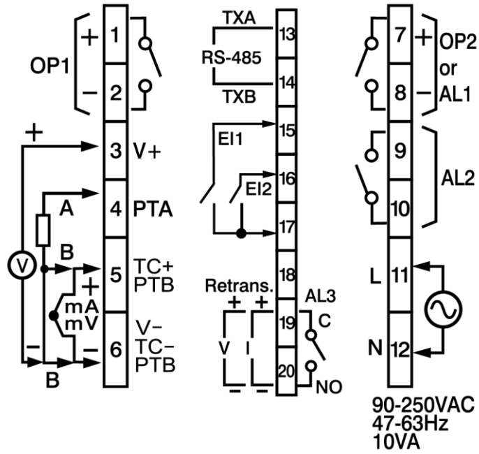
2-9 ZEL-L62 Rear Terminal Connection – High Voltage Input Power
