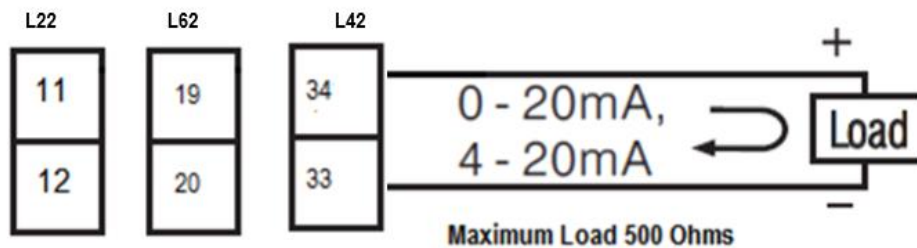
2-24 Retransmission Wiring - Current
