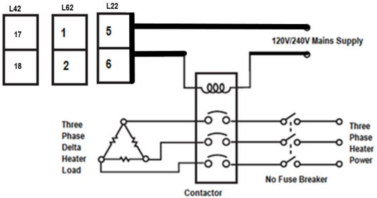
2-18 Output 1 Relay to Drive Contactor
