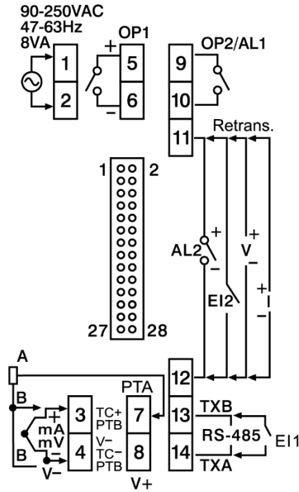
2-11 ZEL-L22 Terminal Connection– High Voltage Input Power
