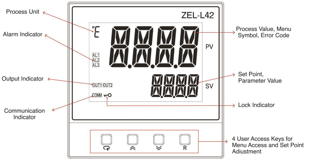
1-3 ZEL-L42 Front Panel Keys and Display
