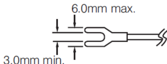
2-6 Lead Terminal
