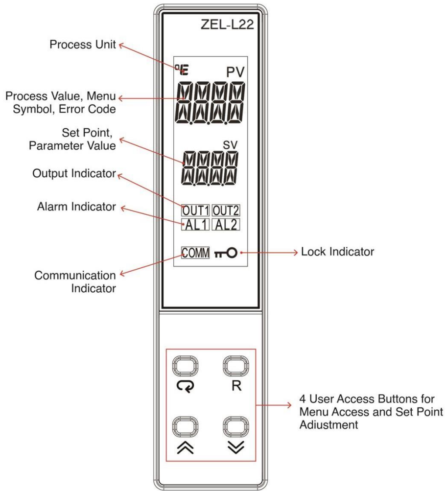
1-5 ZEL-L22 Front Panel Keys and Display
