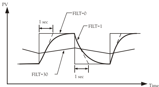
Figure 3.8 Filter Characteristics
