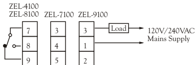
Figure 2.19 Alarm Output to Drive Load
