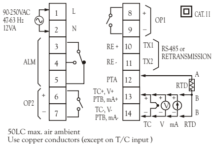
Figure 2.5 Rear Terminal Connection for ZEL-7100
