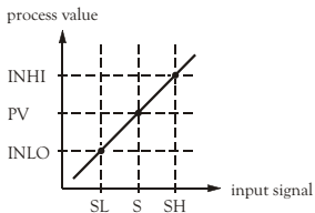
Figure 3.1 Conversion Curve for Linear Type Process Value
