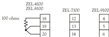
Figure 5.1 RTD Calibration
