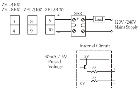
Figure 2.11 Output 1 Pulsed Voltage to Drive SSR
