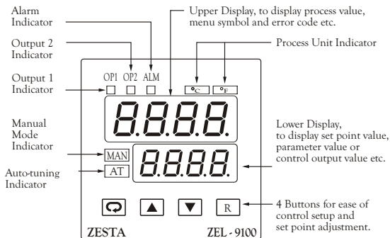
Figure 1.3 Front Panel Description
