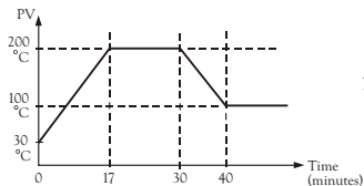
Figure 3.5 RAMP Function
