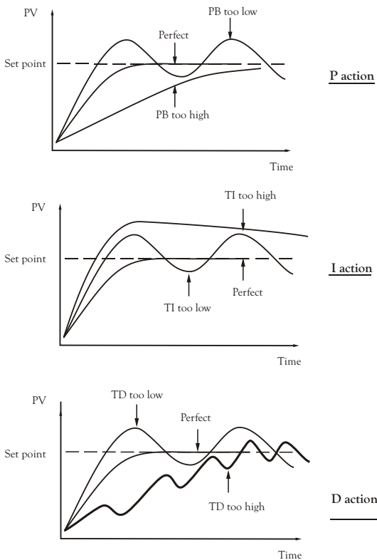
Figure 3.9 Effects of PID Adjustment
