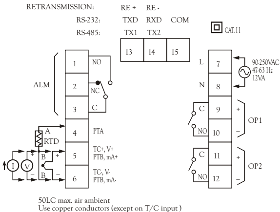
Figure 2.6 Rear Terminal Connection for ZEL-9100
