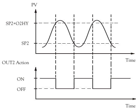
Figure 3.4 Output 2 Process Low Alarm
