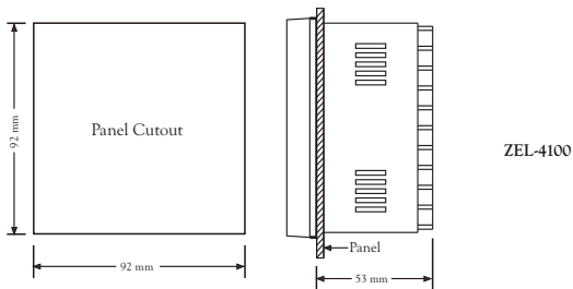
Figure 2.1 Mounting Dimensions
