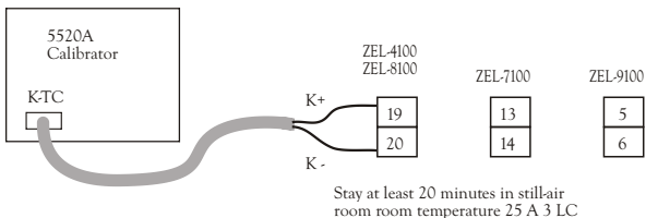
Figure 5.2 Cold Junction Calibration Setup
