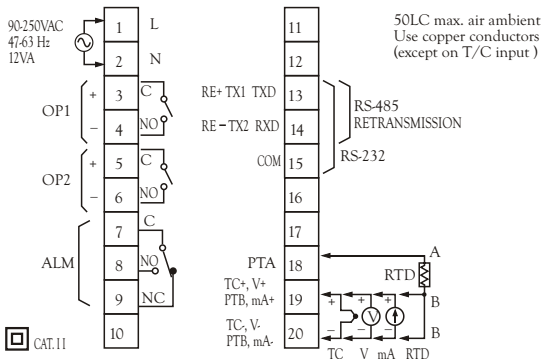
Figure 2.4 Rear Terminal Connection for ZEL-4100 and ZEL-8100
