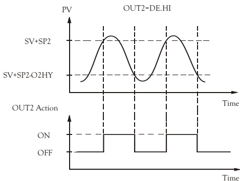
Figure 3.3 Output 2 Deviation High Alarm
