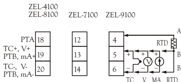
Figure 2.8 Sensor Input Wiring
