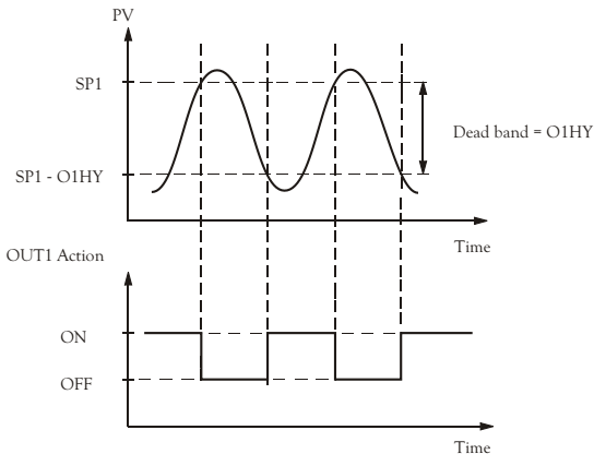
Figure 3.2 Heat Only ON-OFF Control
