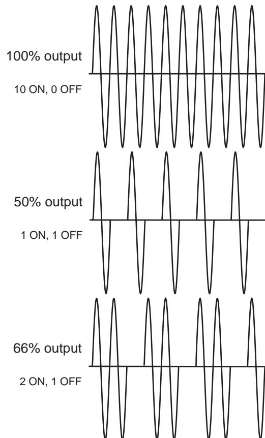
Figure 7.8b — Burst Fire.
