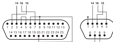
Figure 8.12c — EIA/TIA-232 Connections
