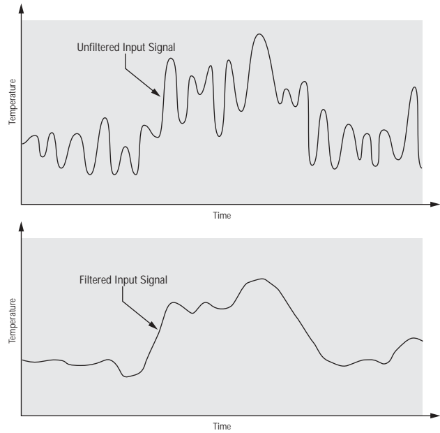
Figure 7.3a — Filtered and Unfiltered Input Signals.
