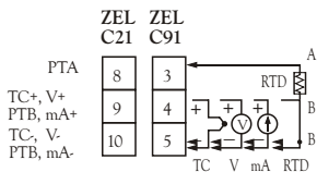
Figure 2.8 Sensor Input Wiring
