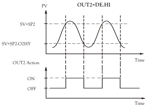
Figure 3.3 Output 2 Deviation High Alarm
