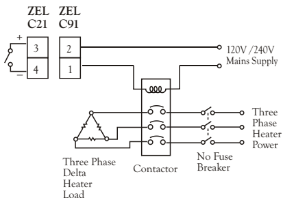
Figure 2.15 Output 2 Relay or Triac (SSR) to Drive Contactor
