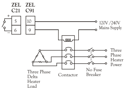
Figure 2.10 Output 1 Relay or Triac (SSR) to Drive Contactor
