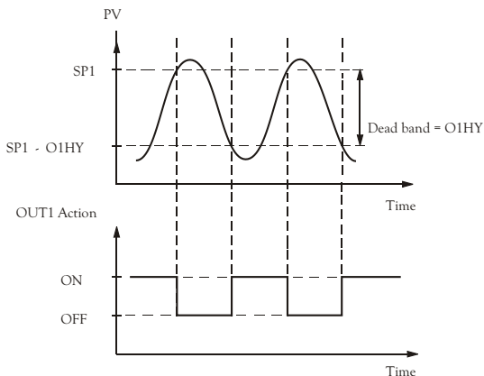
Figure 3.2 Heat Only ON-OFF Control
