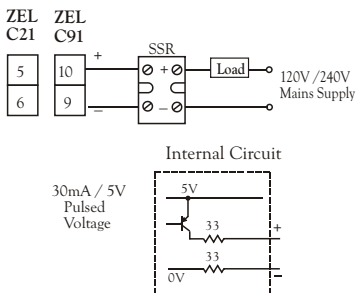
Figure 2.11 Output 1 Pulsed Voltage to Drive SSR
