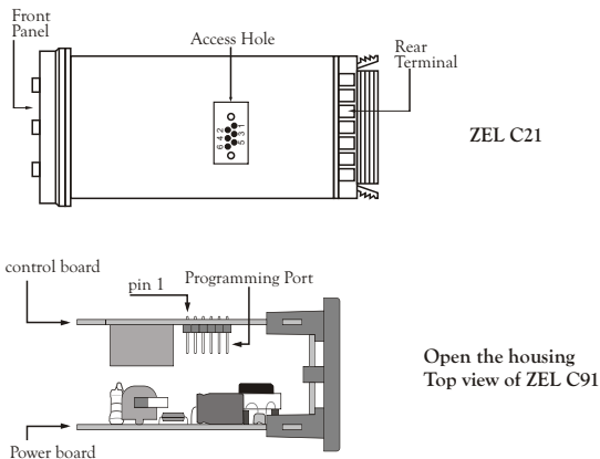
Figure 1.2 Programming Port Overview
