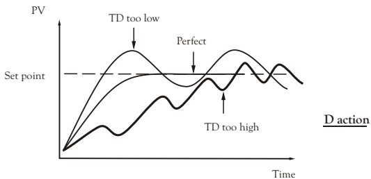
Figure 3.9 Effects of PID Adjustment
