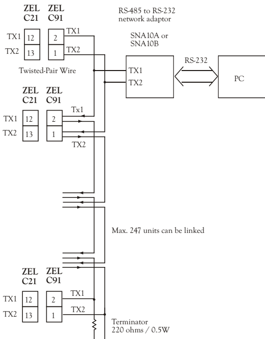
Figure 2.21 RS-485 Wiring
