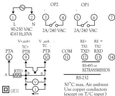
Figure 2.4 Rear Terminal Connection for ZEL C21
