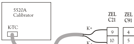
Figure 5.2 Cold Junction Calibration Setup
