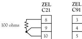
Figure 5.1 RTD Calibration
