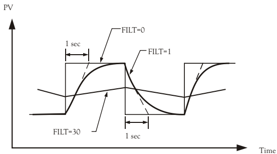
Figure 3.8 Filter Characteristics
