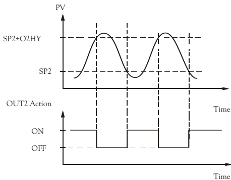
Figure 3.4 Output 2 Process Low Alarm
