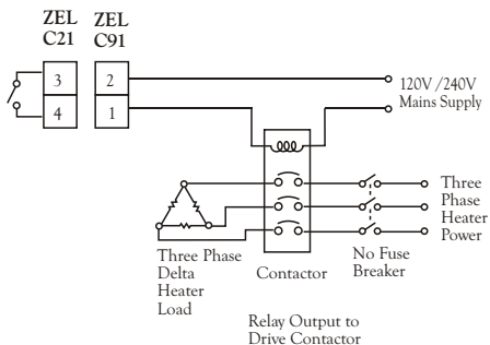
Figure 2.20 Alarm Output to Drive Contactor
