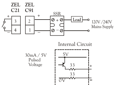
Figure 2.16 Output 2 Pulsed Voltage to Drive SSR
