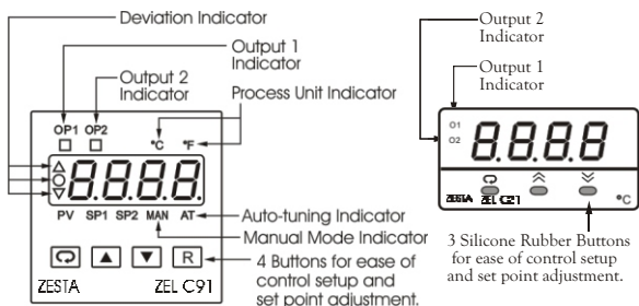
Figure 1.3 Front Panel Description
