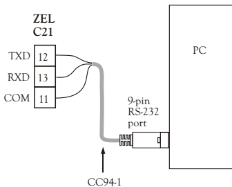
Figure 2.22 RS-232 Wiring
