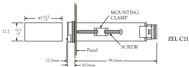
Figure 2.1 Mounting Dimensions
